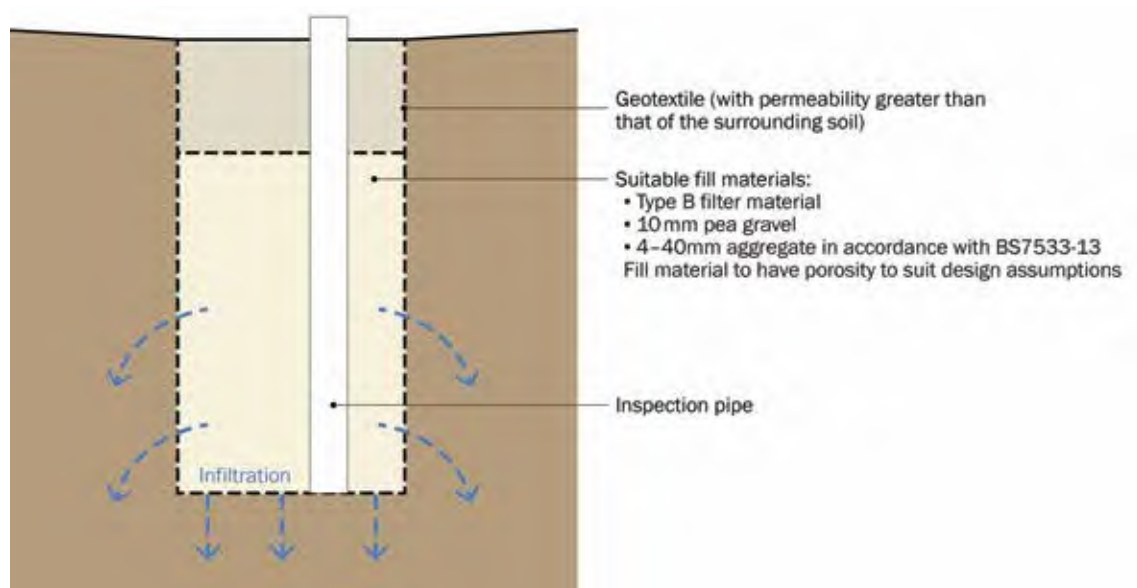
Figure 13.3 Infiltration trench
